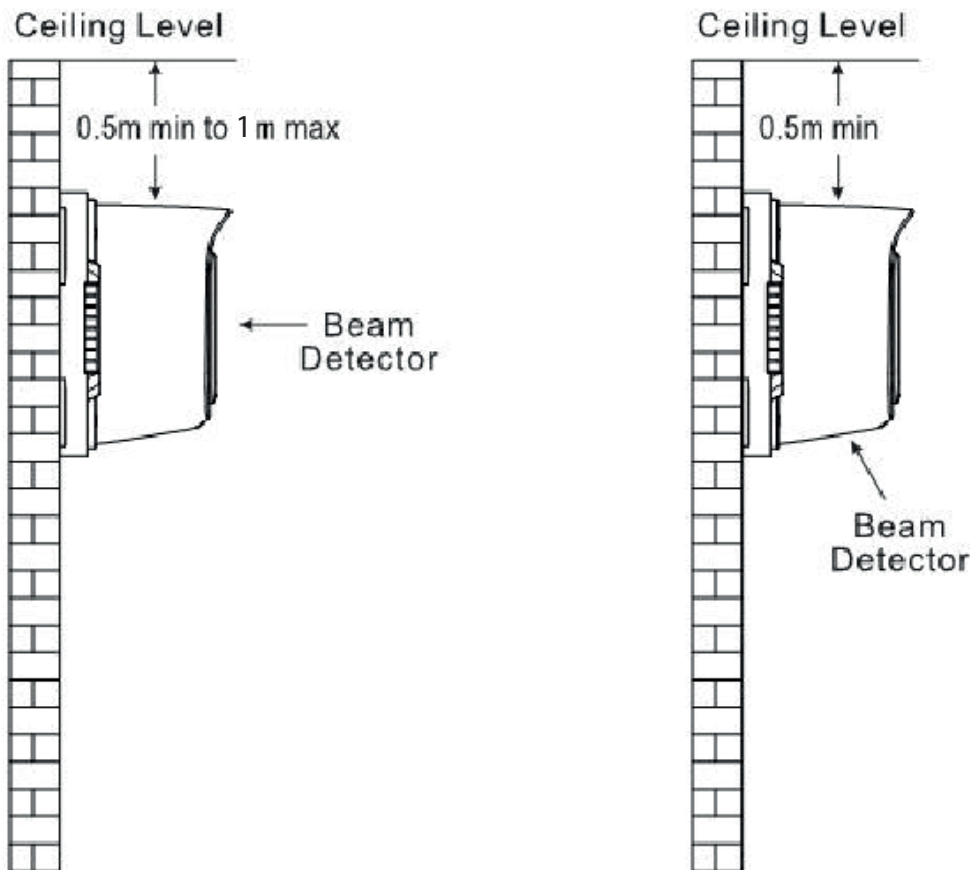
Figure 3: Installation Details
